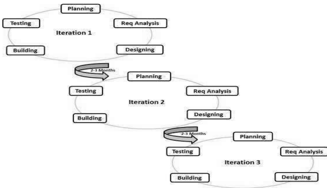
Figure 10: Agile Model
